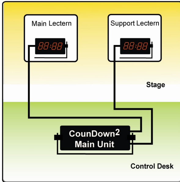
Figure 1 Connections Diagram
